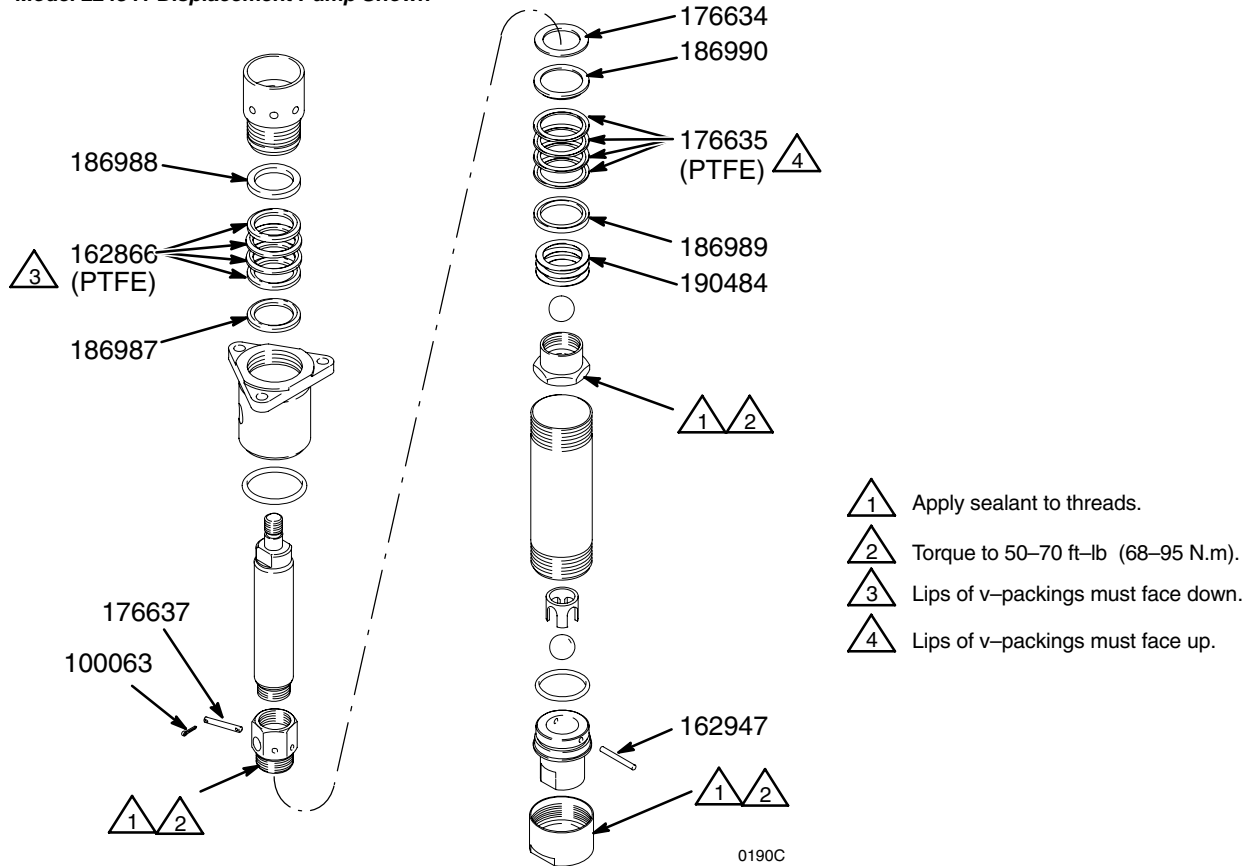
Model 224341 Displacement Pump Shown
