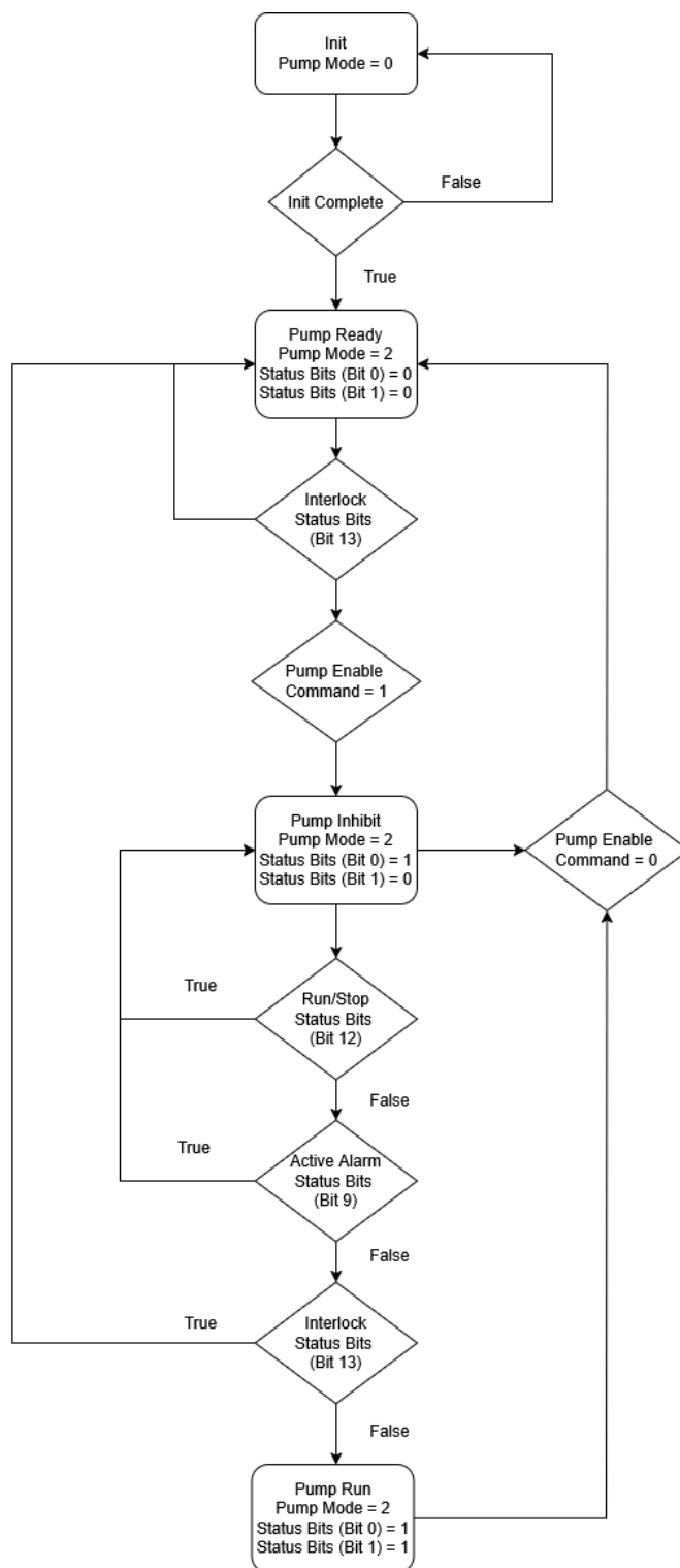
FIG. 47: Sequence of Operation
