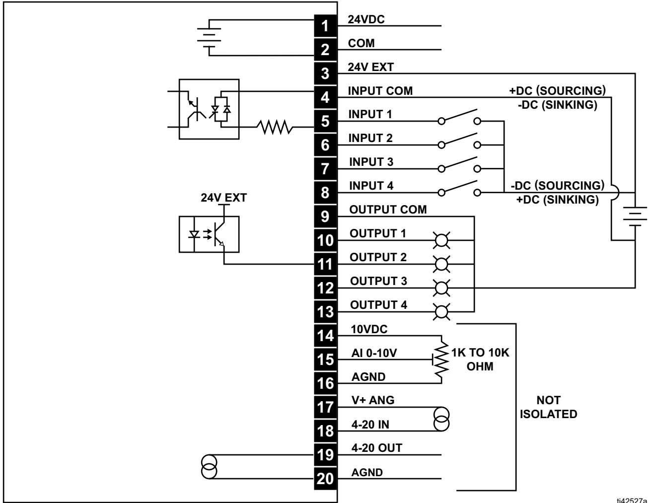
FIG. 12: Isolated Sinking I/O with External 24 vDC Power Supply
