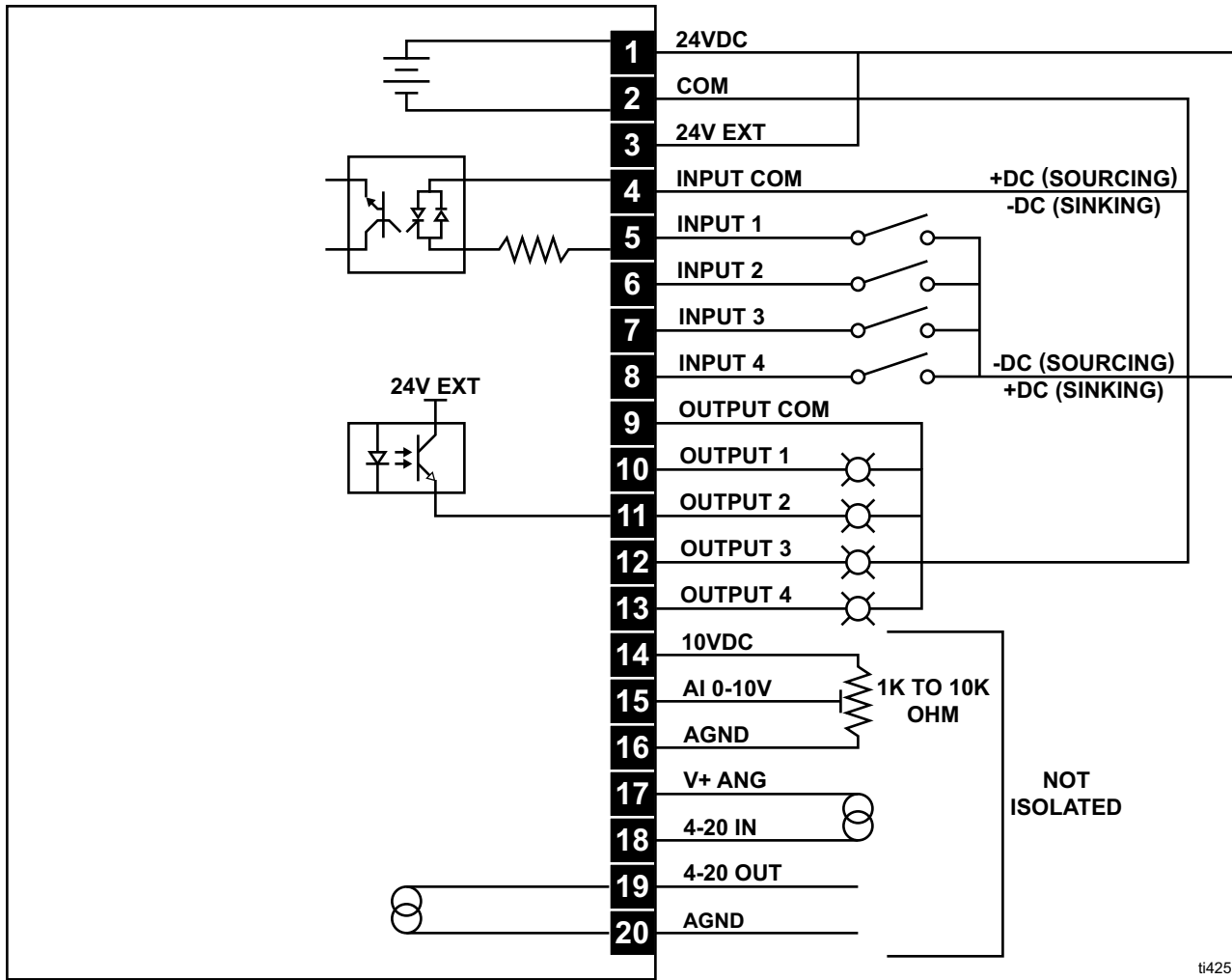
FIG. 15: Sinking I/O with Internal 24 vDC Power Supply
