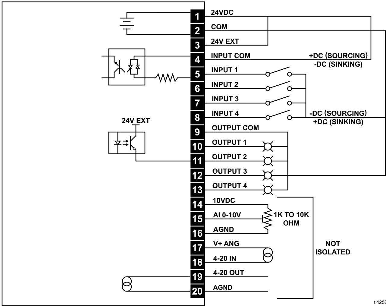
FIG. 14: Sourcing I/O with Internal 24 vDC Power Supply
