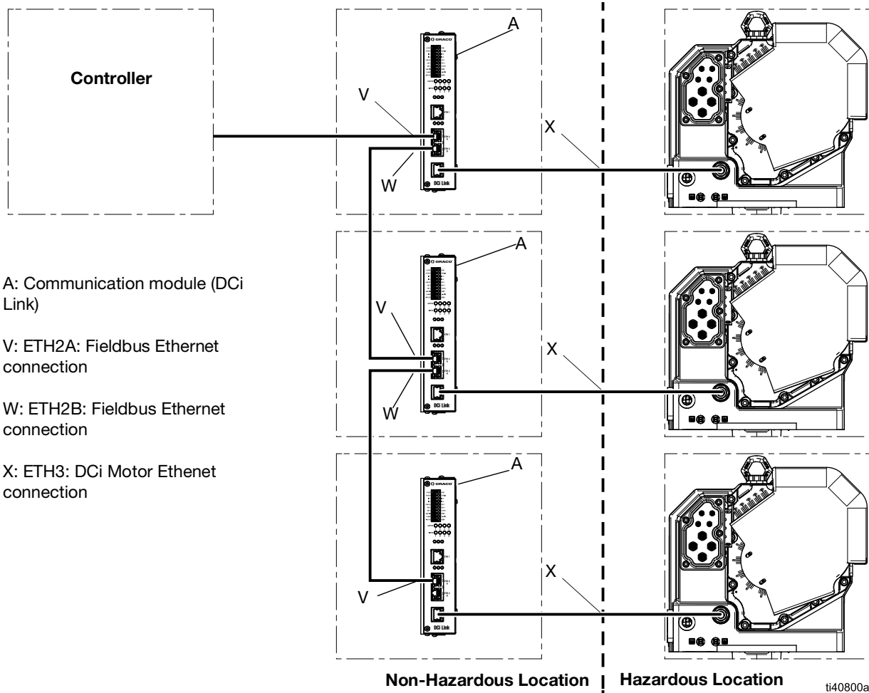
FIG. 9: Daisy chain installation
