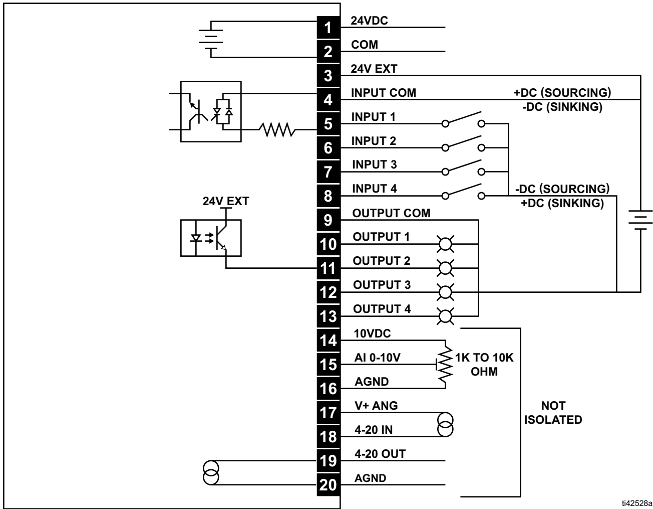
FIG. 13: Isolated Sourcing I/O with External 24 vDC Power Supply
