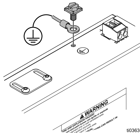
ti03630a Fig. 4: Ground Screw
