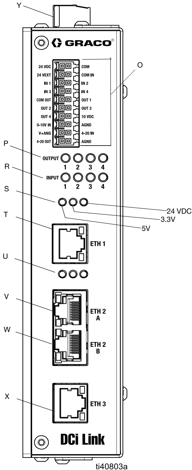
FIG. 10: Front Connections
