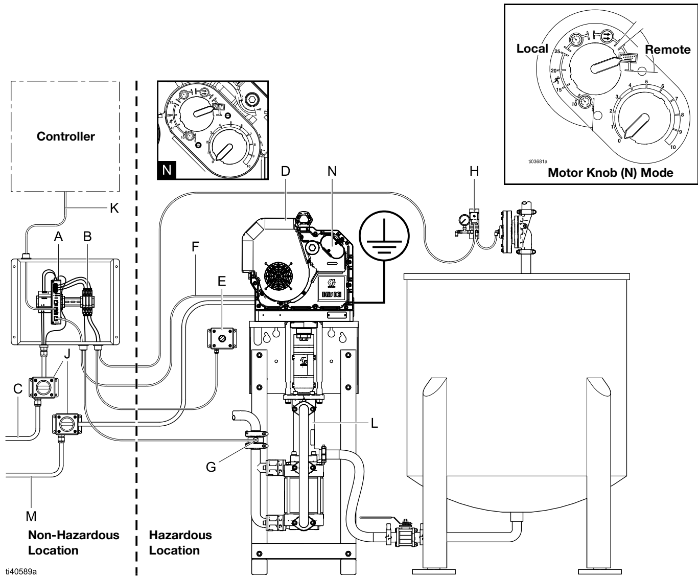
FIG. 2: Typical Installation
