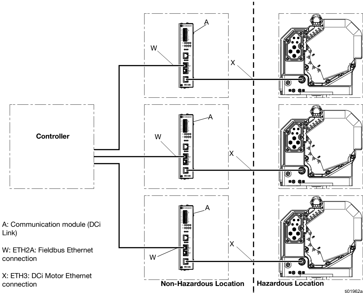
FIG. 8: Point-to-Point installation
