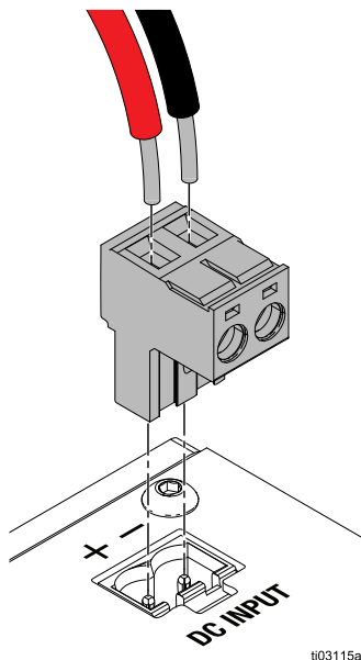
FIG. 5: DC Power Connector
