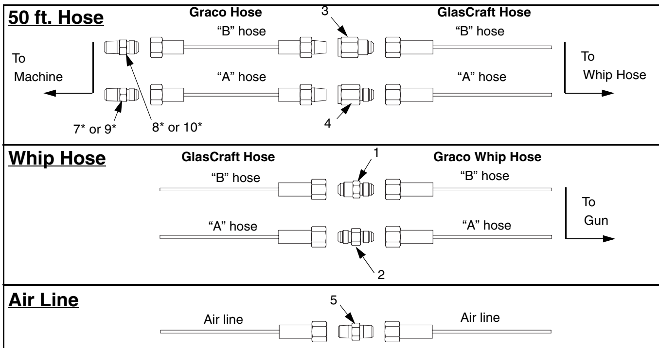
FIG. 1: Connect Graco and GlasCraft Hoses
