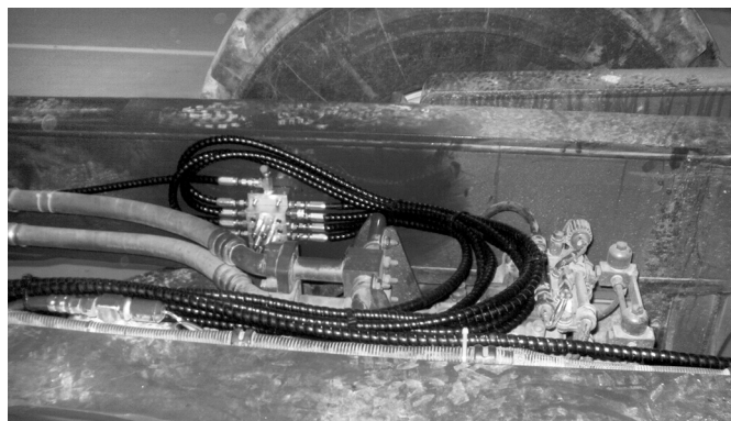
FIG. 109: Lubrication hoses routed across dump bed to Middle Secondary Divider Valve installed inside of the right side dump body frame rail on HM300-5.
