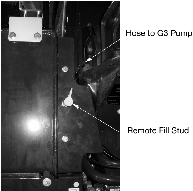
FIG. 51: Remote Fill Stud installed on HM300-5
