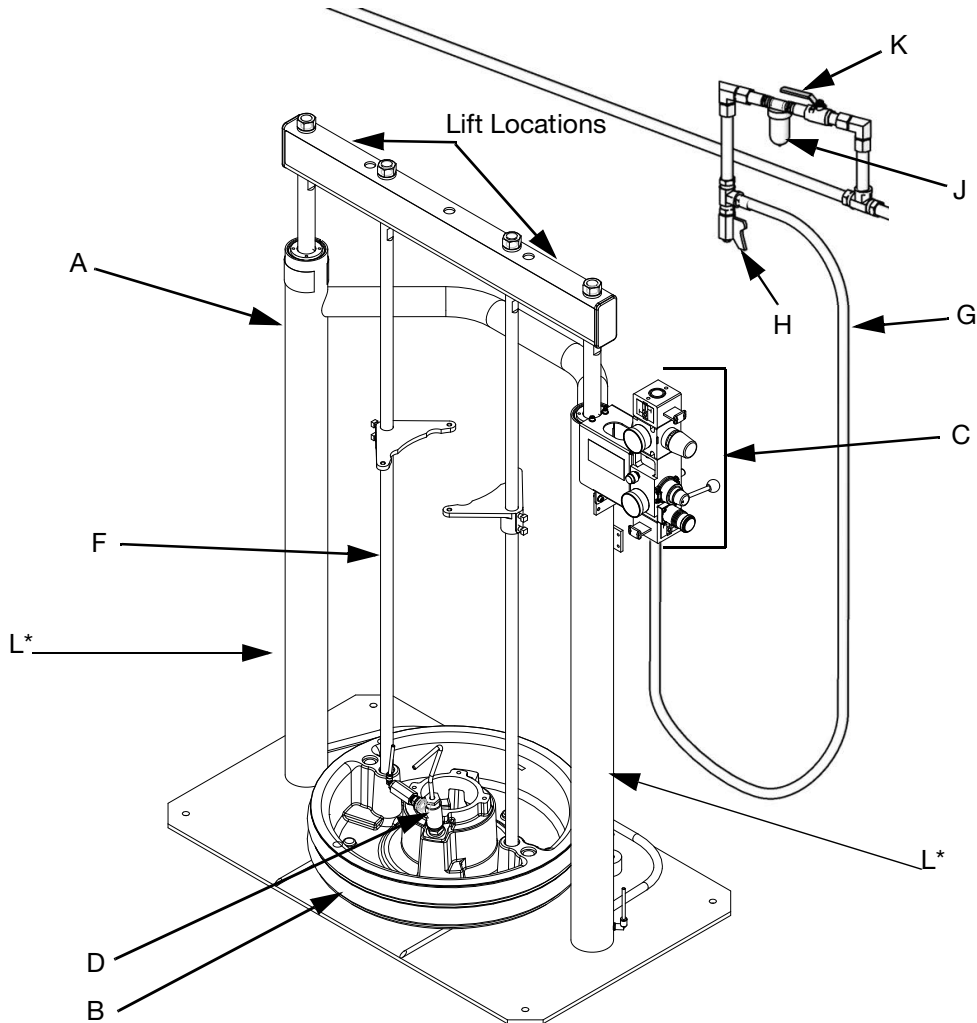
FIG. 1: Typical Installation
