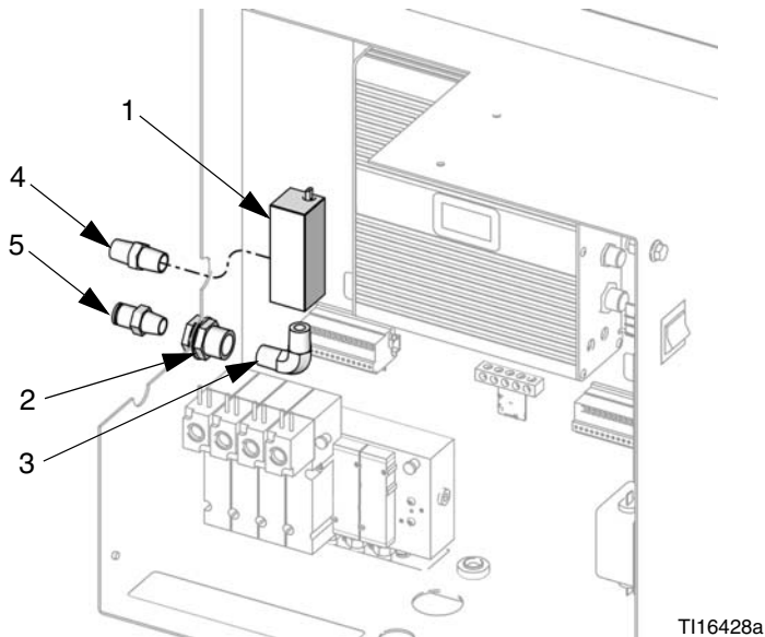
Install Air Flow Switch in Control Box
