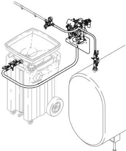
Package 224873 installed on Oil King and tank (neither included in package).
