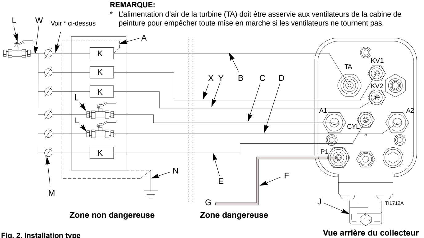
Fig. 2. Installation type
