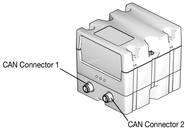
Fig. 4: CGM Connectors
