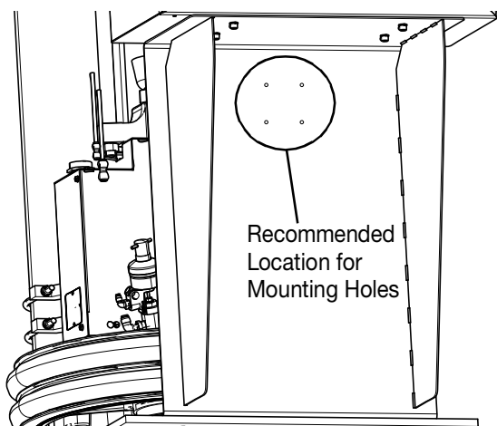
FIG. 1: Mounting Location
