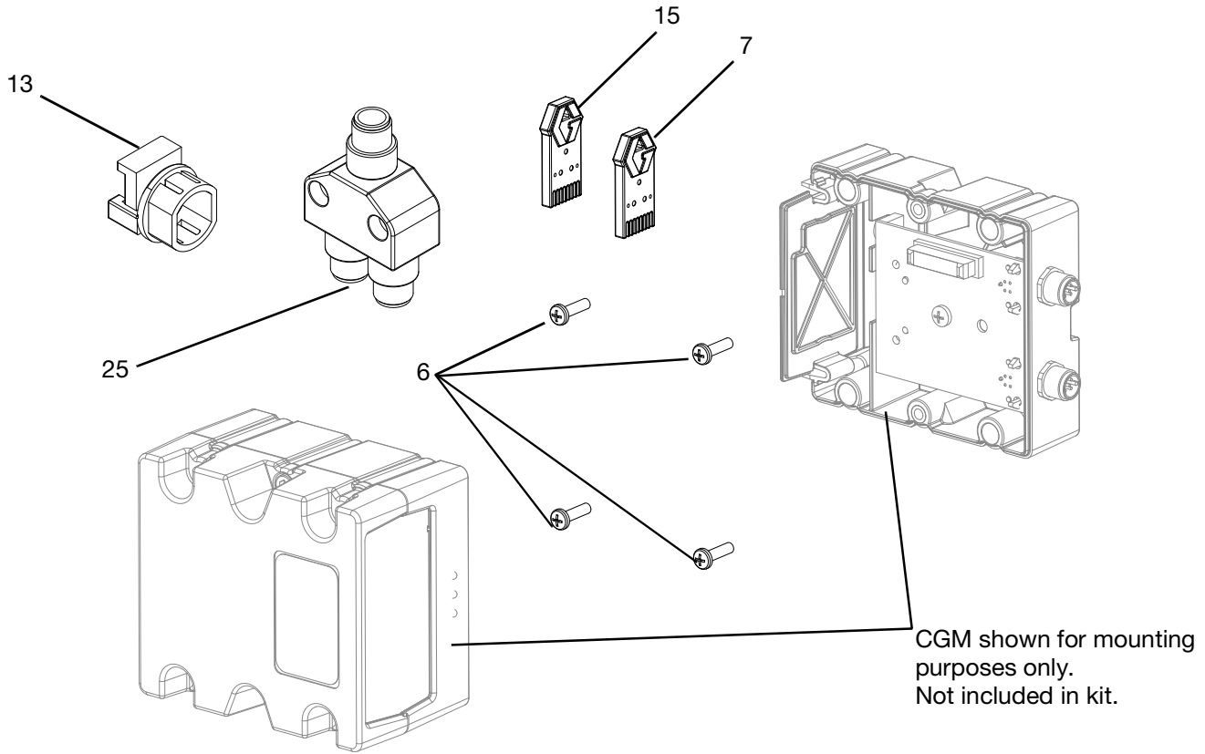
FIG. 7: Kit 25C994 Parts
